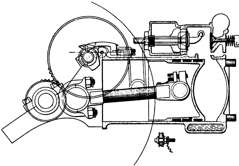
FIG. 301.—Sectional View through one Cylinder of the Duryea Carriage Motor, showing working parts. The exhaust cam operated by a 2 to 1-gear system from the main shaft, imparts a double motion to the valve pushrod; a lift for opening the valve, and a double twist for making and breaking the connections of the electrical spark. The valve and sparking chamber is projected so as to show the position of contained mechanism on a plane different from that of the cylinder section. Details of the insulated sparking anvil are shown below the cylinder. It is an iron contact point, having a mica washer on the inside and the outside of the cylinder walls, and a mica bushing between, so as to perfectly insulate it from the metal of the engine. A very short water jacket and the concave cylinder and piston heads are also exhibited in this figure.
